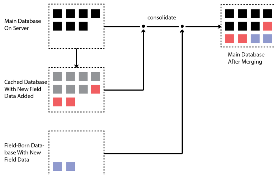
Figure 2, A database merging mechanism. Offline field capture data is stored in a cached database (red) or a new field-born database (blue), and reintegrated with the main database after the field work.
